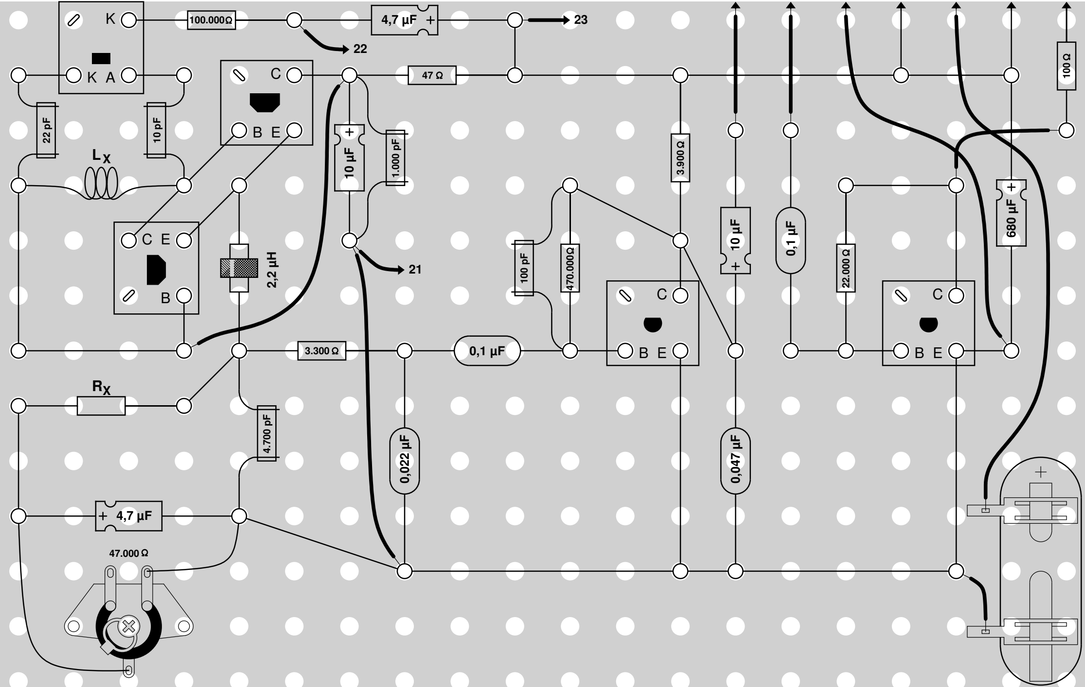
Superregenerative FM receiver
